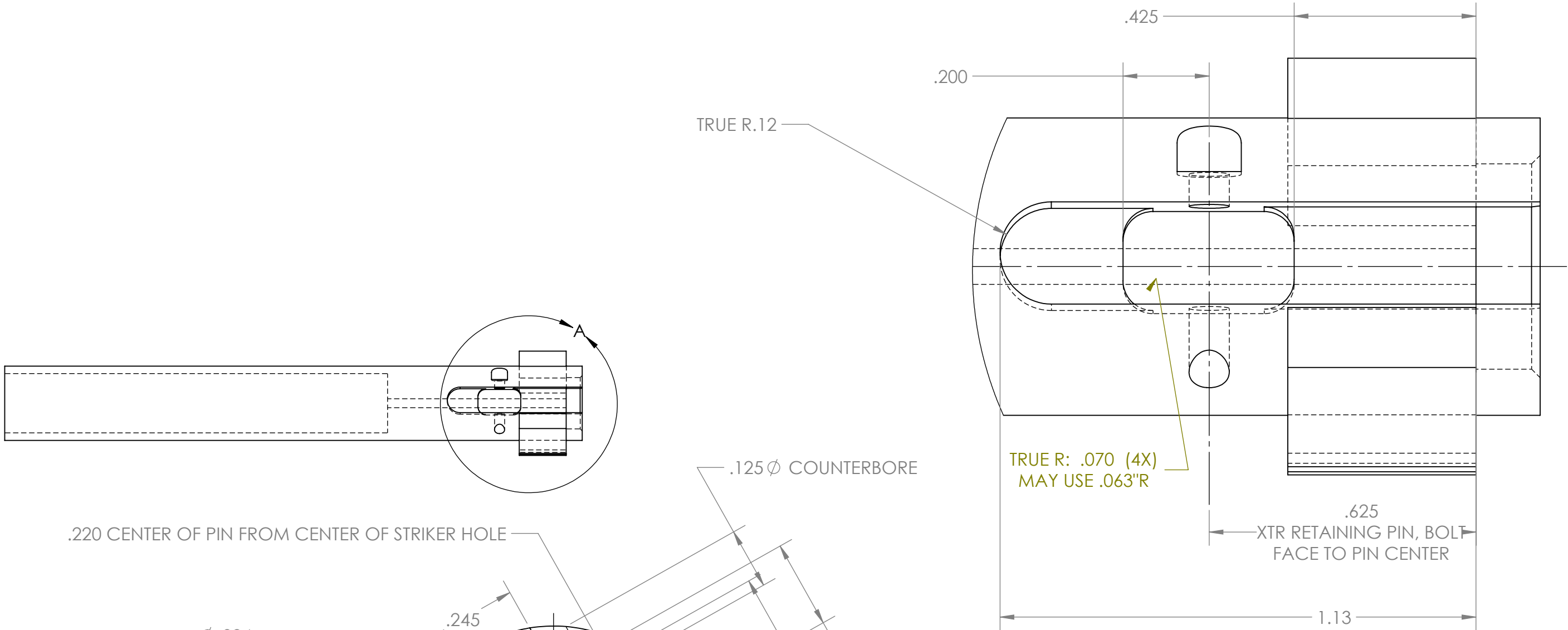
DETAIL A SCALE 4 : 1
